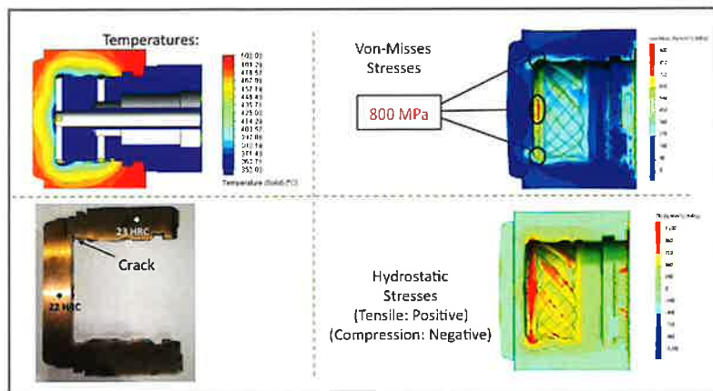
Fig. 1 Failure analysis of a cracked copper-beryllium plunger tip
