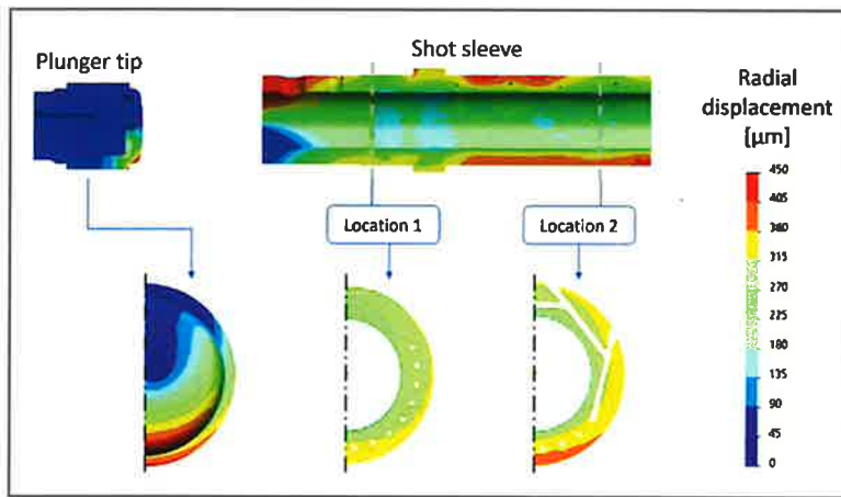
Fig.2 Simulation results showing the radial displacement/deformation in shot sleeve and plunger rod during the process
