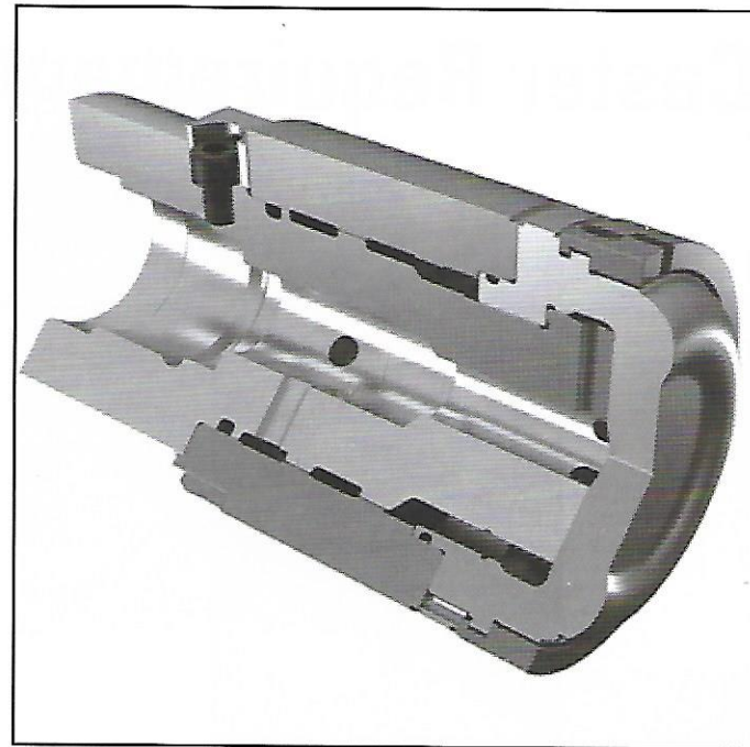
AMP-R with Con Duct head designed for 120 to 200 mm dia
