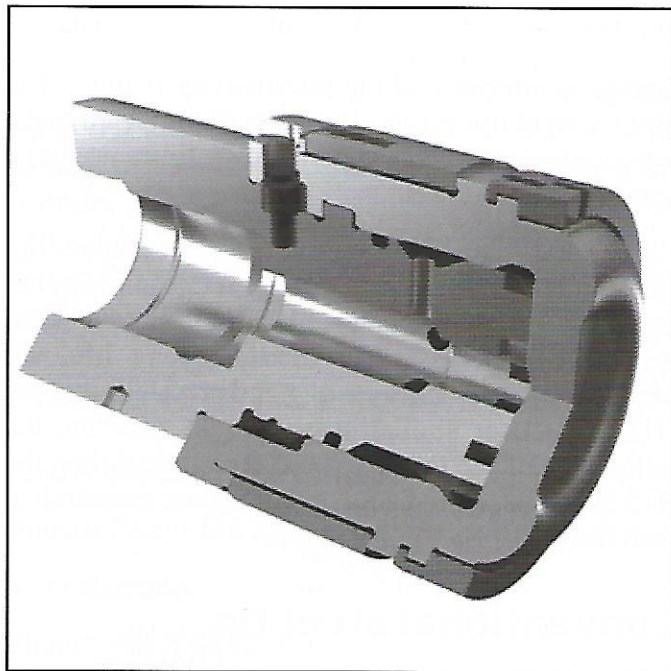
ABP-R with Con Duct body designed for 50 to 120 mm dia
