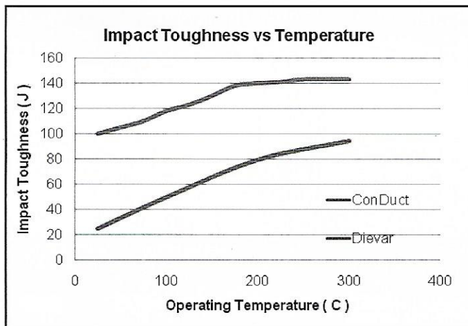
Figure 2. Impact toughness of ConDuct and Dievar steels
