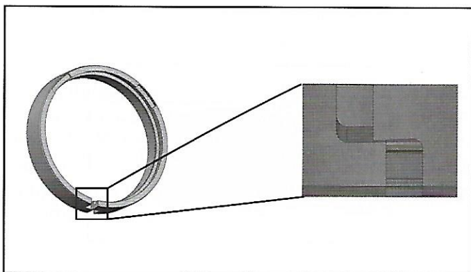
Figure 3. anitrided split ring made of H13 to provide excellent wear resistance on tip
