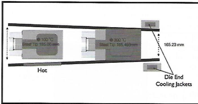
Figure 1. The plunger tip over expands and sleeve contracts near die end.
